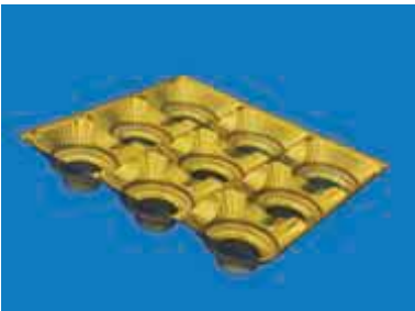
84319 9 Cell Tray O.D.: 5.750 x 5.750 x 0.875 I.D.: 1.375 x 1.375 x 0.625 Mat.: OPS, HIPS
